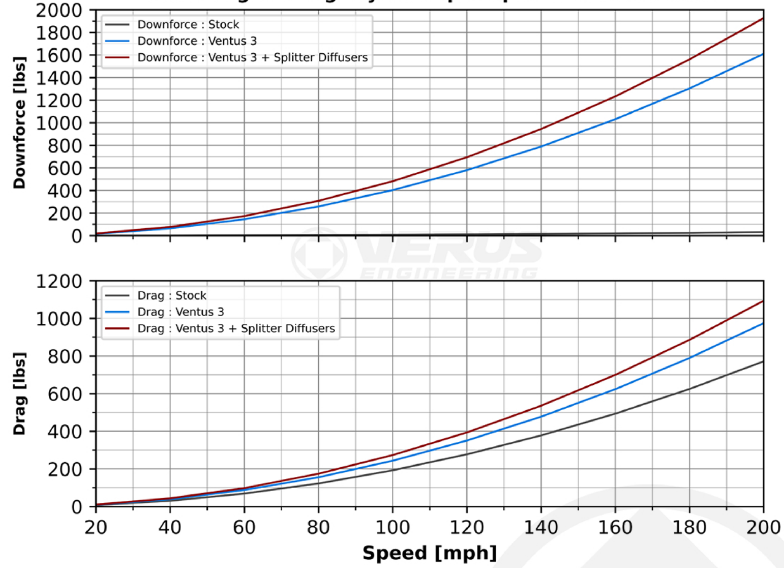
Verus Engineering Toyota Supra Splitter Diffuser Data
